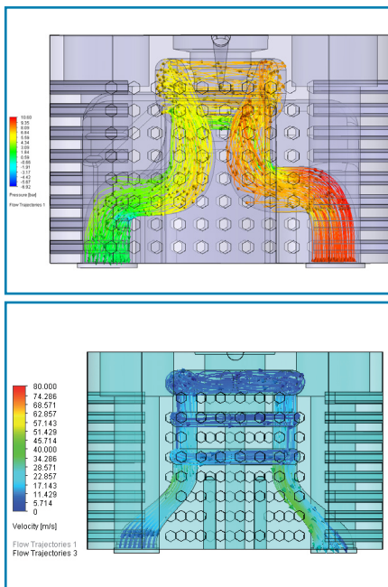
Fluidodynamik-CFD-Simulation
